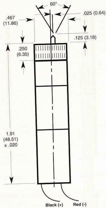
BMP-1 For use in Series 32 G-10 fixtures Patent Pending
