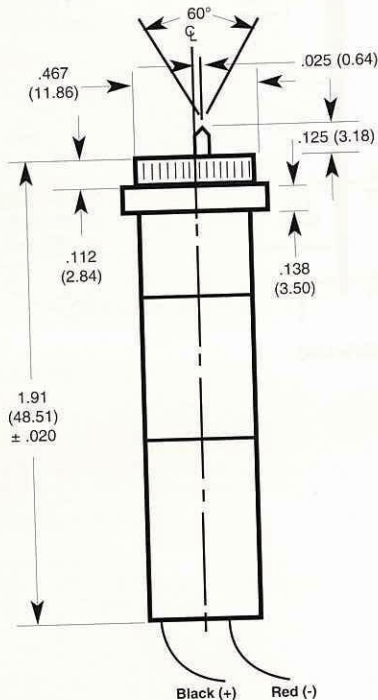
BMP-2 For use in Lexan Drop Pin Fixtures Patent Pending
